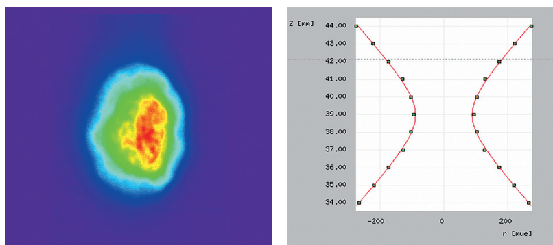
Measuring a caustic with the FPM (Optional Interface to the external z-axis is necessary)
